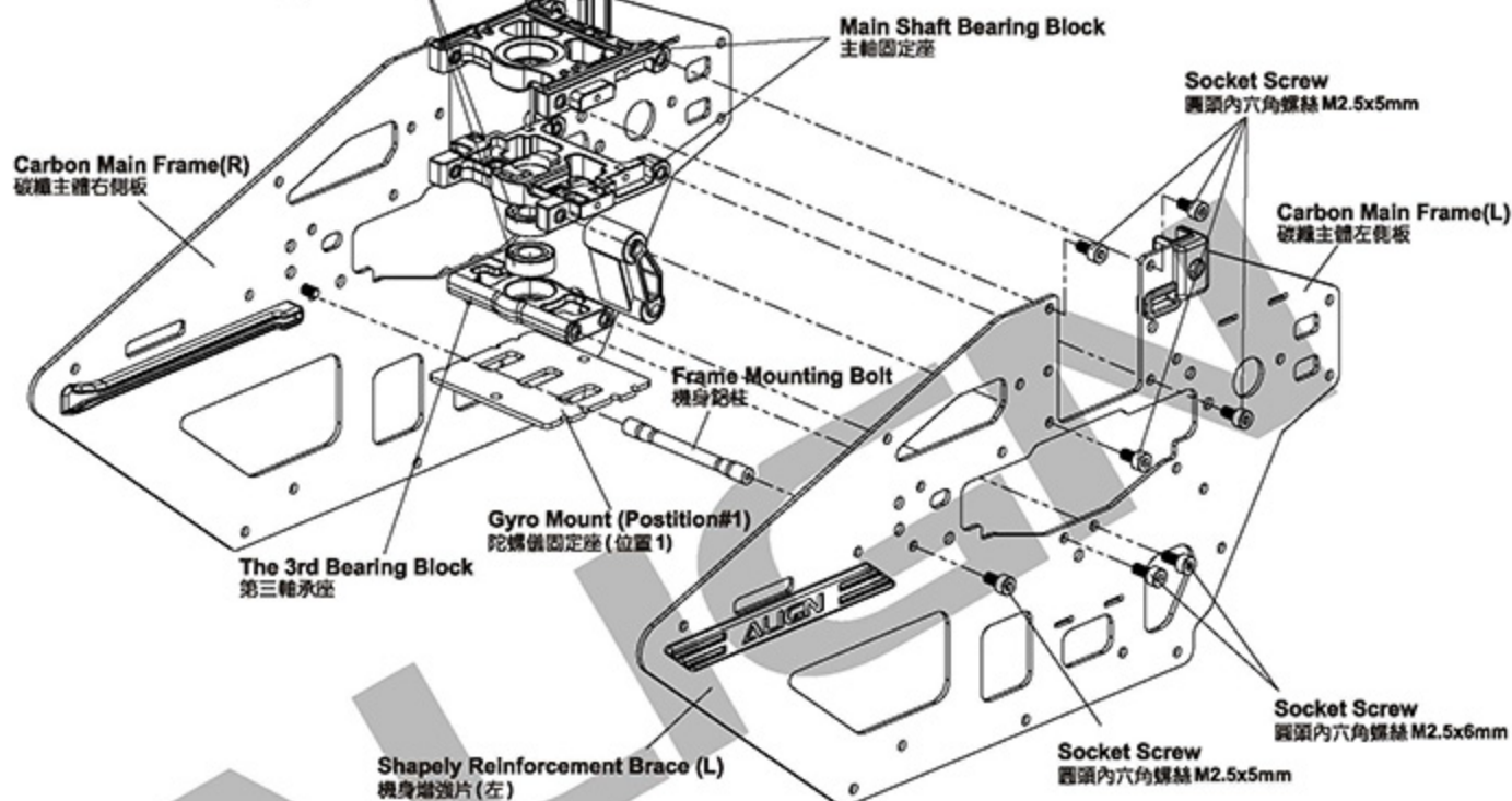
Socket Screw 圓頭內六角螺絲 (M2.5x6mm) x 4
