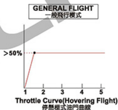
Governor Function Throttle Settings Instruction 定速模式油門曲線設定圖
