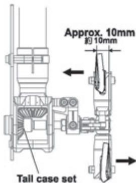
Tail case set 尾齒輪組
